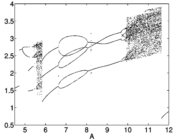
FIG. 2. Bifurcation diagram for system (12). At A \approx 6.6 and A \approx 8.0 a period-3 limit-cycle undergoes supercritical and subcritical pitchfork bifurcations, respectively. This is a signature of symmetry in the system.
