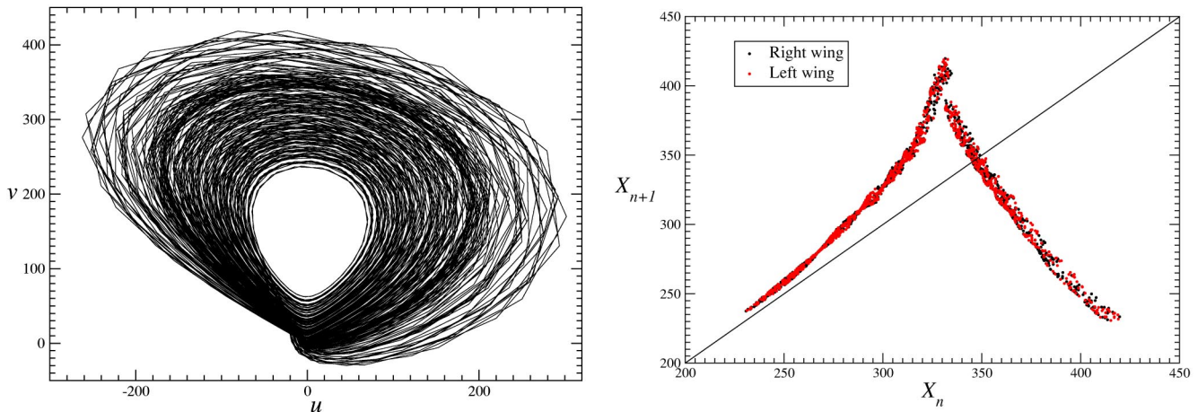
FIG. 11. Results obtained with a RBF network trained from symmetrical data but with no symmetry constraints whatsoever. (a) Image of the attractor, (b) first-return map on which the data on the left and right wings are very difficult to distinguish.
