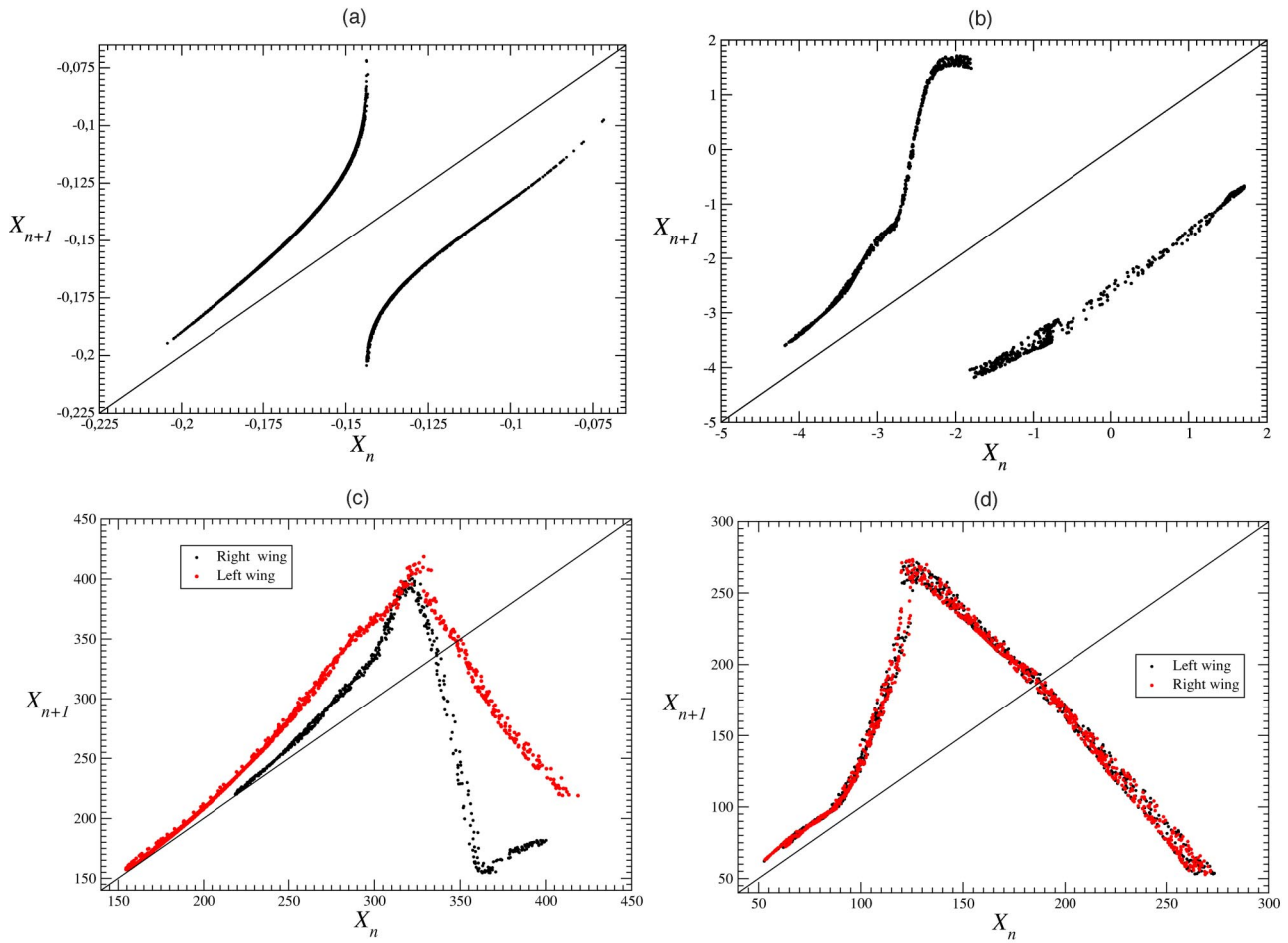
FIG. 9. First-return maps to a Poincaré section for (a) the asymmetric avatar of the Lorenz system and (b)–(d) for the different RBF models obtained. (b) Map computed for a RBF model trained without any constraints, (c) with pairs of symmetrical centers but no constraints on the weights, and (d) with pairs of symmetrical centers and constrained weights.
