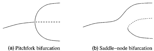
FIG. 4. By adding a simple term, the symmetry of the system is broken. In (a) the original branch loses stability giving birth to two stable branches via a pitchfork bifurcation. In (b) the original branch does not bifurcate at all. The second stable branch appears through a saddle-node bifurcation. Such a scenario is observed in Fig. 3(b) at A \approx 6.6 .
