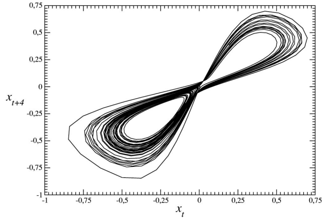
FIG. 8. Avatar of the Lorenz system for which the symmetry is broken. Parameters: (a, b, c, d) = (0.1, 0.07, 0.38, 0.0015) .
