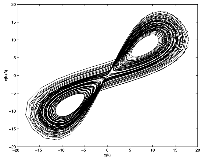
FIG. 6. Bidimensional delay reconstruction of the Lorenz attractor from the x variable. This reconstructed attractor has an inversion symmetry.
