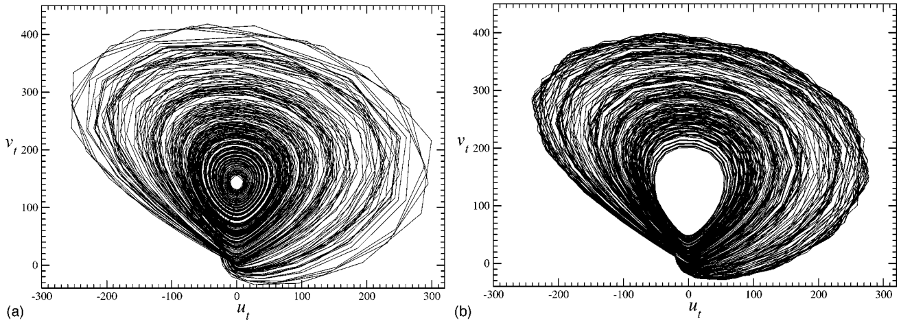
FIG. 10. Image of the attractors of the RBF model trained (a) with pairs of symmetrical centers but no constraints on the weights and (b) with pairs of symmetrical centers and constrained weights.
