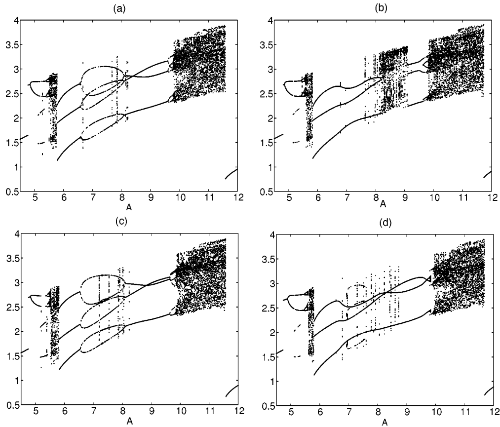
FIG. 5. Bifurcation diagrams of networks (a) HHHLL, (b) HHHLLB, (c) HHHHL, and (d) HHHHLB. Cases (a) and (c) correspond to networks without any bias terms and cases (b) and (d) to networks with bias terms.
