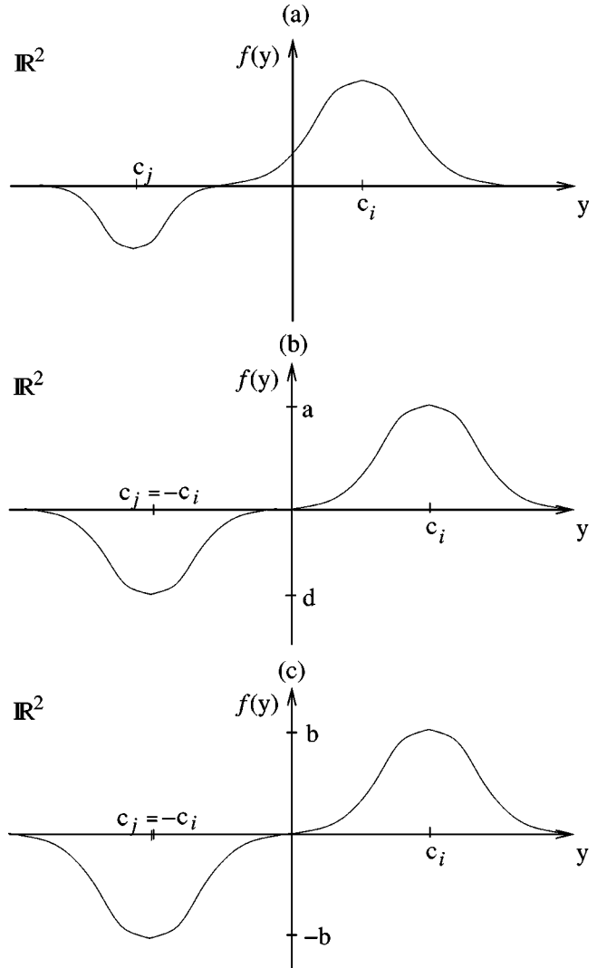
FIG. 1. Schematic illustration of how symmetry can be imposed during training of a RBF network. In (a) no restrictions are imposed, and in (b) the centers are taken to be symmetrical with respect to the embedding space but no restrictions on the weights are used. Finally, in (c) besides taking symmetrically spaced centers, the weights of each pair of symmetrical centers are constrained to be such that \omega_i = -\omega_j . Clearly, only in (c) is the function f(y) odd.
