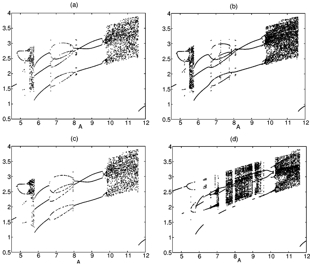
FIG. 3. Bifurcation diagrams of networks (a) HLL, (b) HLLB, (c) HHL, and (d) HHLB. Cases (a) and (c) correspond to networks without any bias terms and cases (b) and (d) to networks with bias terms.
