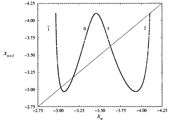
FIG. 3. First-return map of the simplest equivariant chaotic system just before the attractor merging crisis ( \alpha = 2.027\ 717 ).
