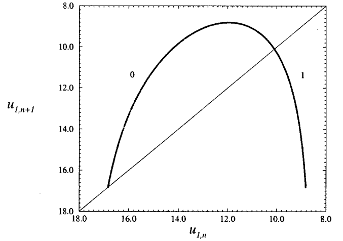
FIG. 5. First-return map of the image system of the simplest equivariant chaotic system just before the attractor merging crisis ( \alpha=2.027\ 717 ). A similar map may be obtained using the u_3 variable.
