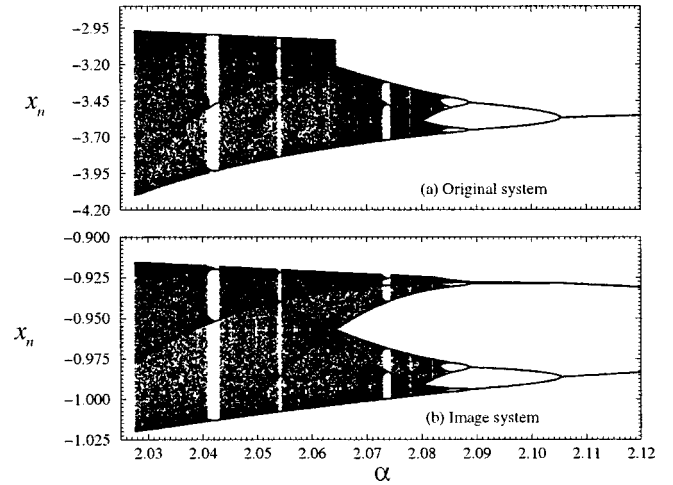
FIG. 2. Bifurcation diagrams versus \alpha for the simplest chaotic dynamics (3) and its image.
