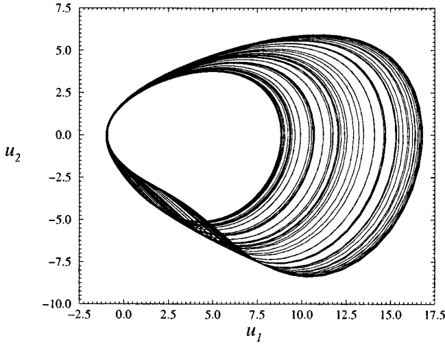
FIG. 4. Image of the simplest equivariant chaotic system just before the attractor merging crisis ( \alpha=2.027\ 717 ).
