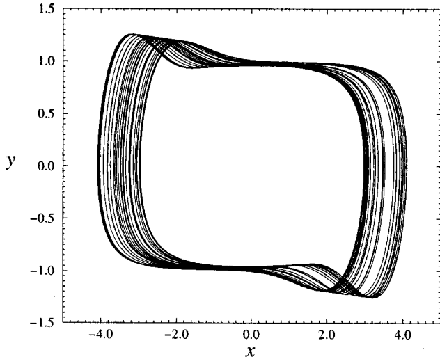
FIG. 1. Chaotic attractor generated by the simplest equivariant chaotic system just before the attractor merging crisis ( \alpha = 2.027\ 717 ).
